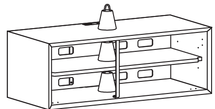
clic 220 Center + support bars = 45kg clic 221 Center + support bars = 45kg clic 222 Center + support bars = 40kg
