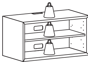
clic 210 Large = 40kg clic 211 Large = 40kg clic 212 Large = 40kg
